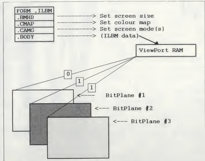
Body data is read a byte at a time into each bitplane.
